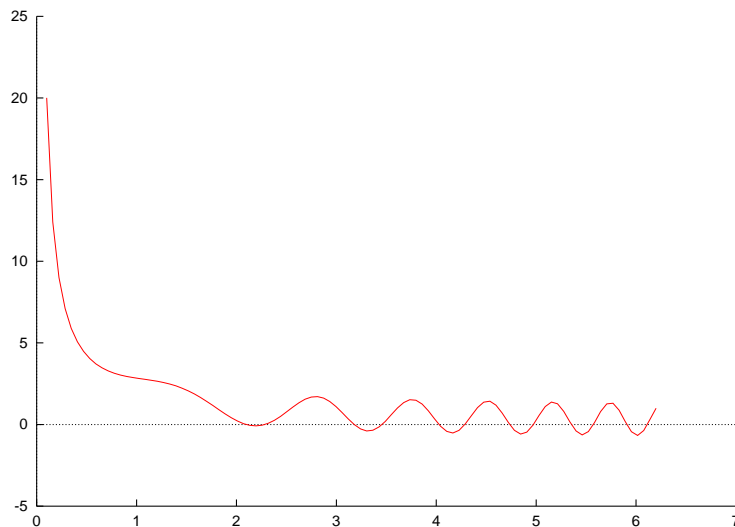
Figure 16.4: Function y(x) = 2/x + \sin(x^2) .
