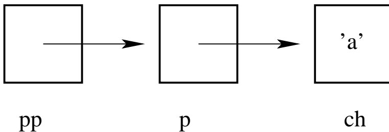
Figure 9.5: Pointer to pointer.
