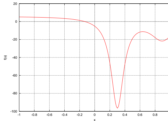
Figure 24.5: Function f(x) = -\frac{1}{(x-0.3)^2 + 0.01} - \frac{1}{(x-0.9)^2 + 0.04} + 6 .
