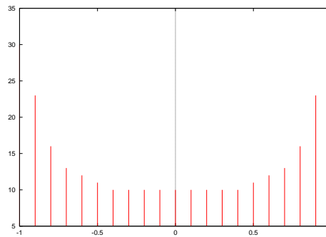
Figure 24.2: The histogram for \sin(x) in the range of -\pi \leq x \leq \pi .
