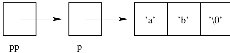
Figure 9.6: Pointer to string.
