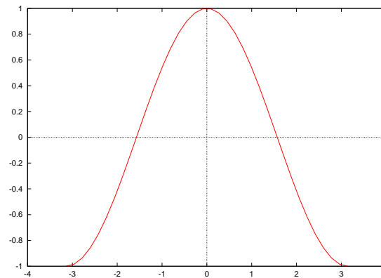
Figure 24.7: The derivatives for \sin(x) in the range of -\pi \leq x \leq \pi .
