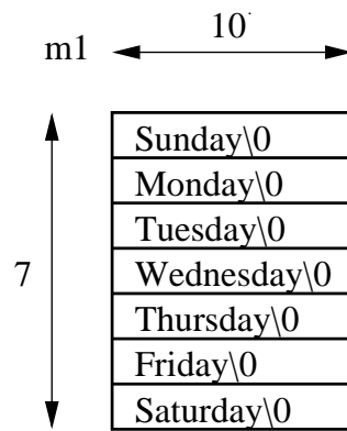
Figure 9.1: 2D array.
