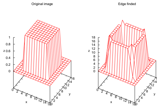
Figure 24.9: The result from two-dimensional convolution function conv2() .
